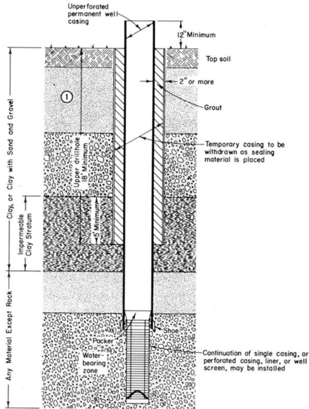
① Unperforated well casing and annular seal must extend at least 5 feet into impermeable stratum, and must extend at least 18 feet below land surface.
