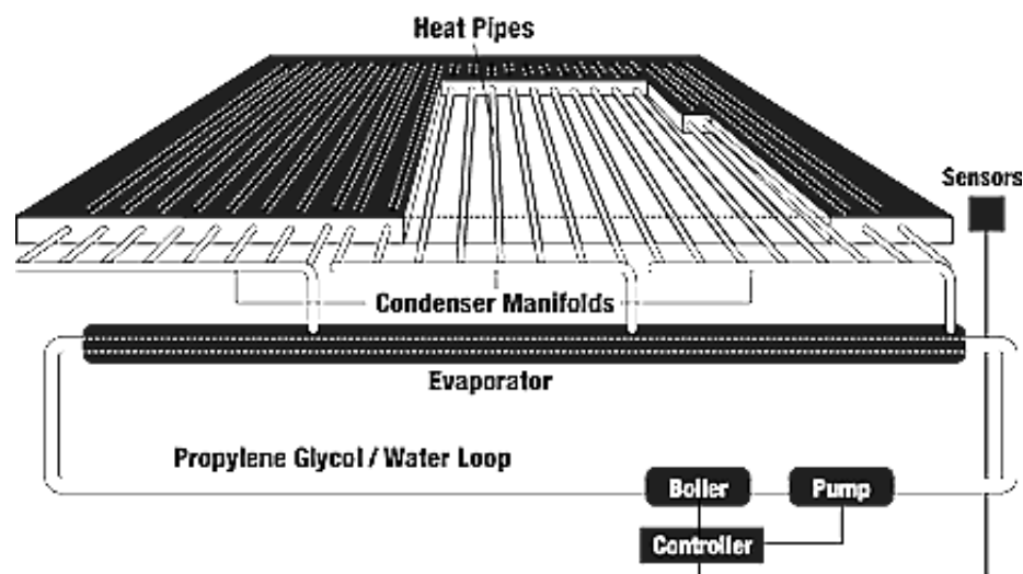
Figure 4. Schematic of the VDOT anti-icing system.
