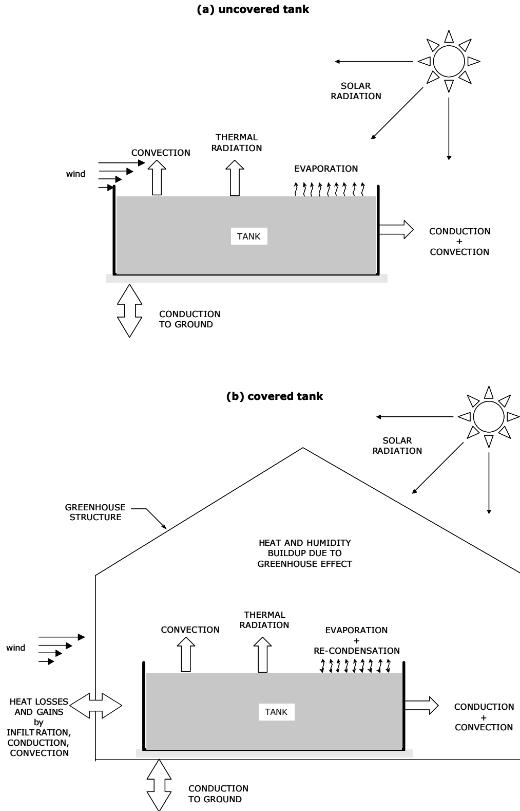
Figure 1. Heat transfer processes in covered and uncovered aquaculture tanks.
