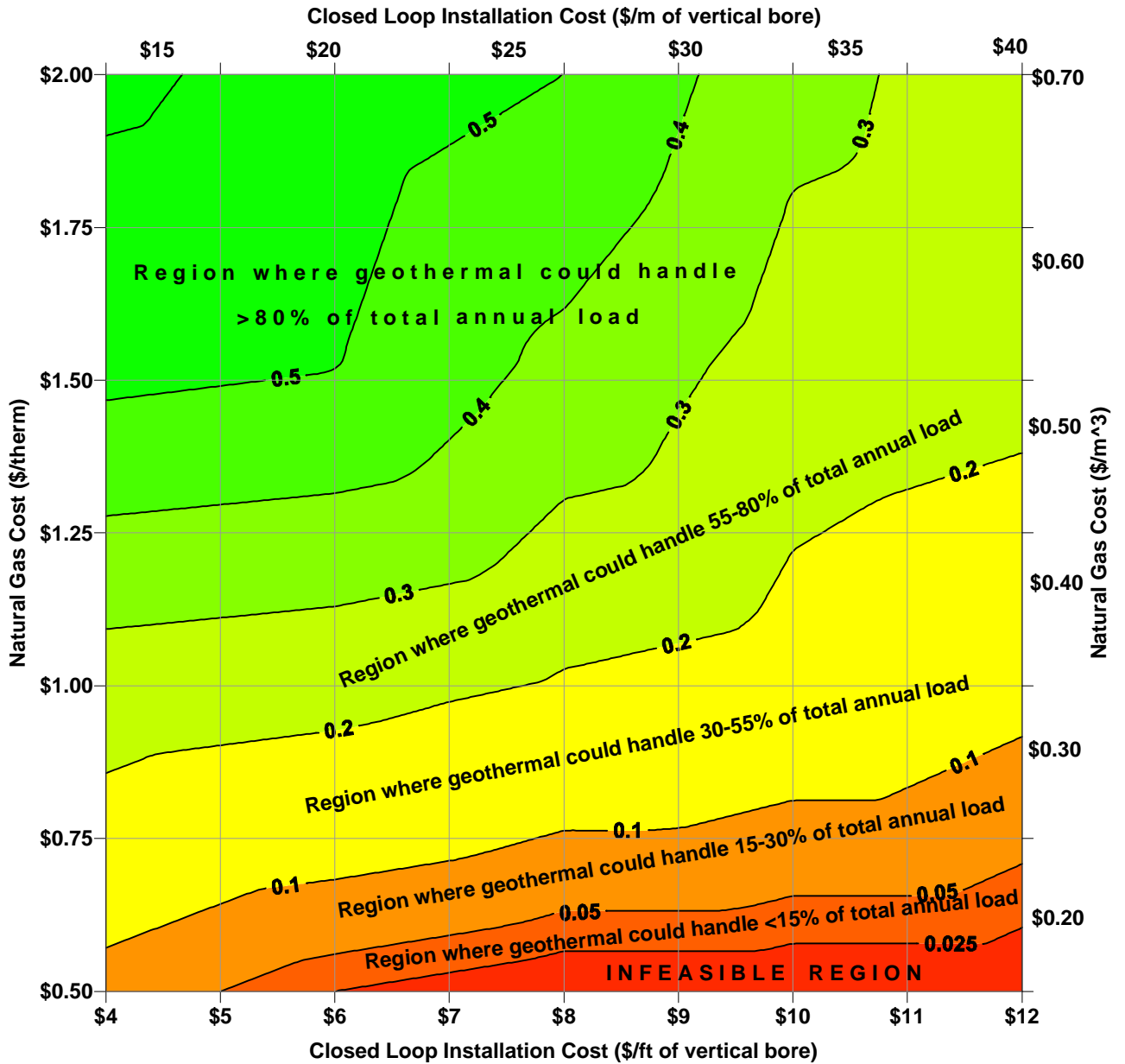
Figure 6. Closed-loop GHP system fraction providing lowest net present value of a 20-year life cycle at various natural gas costs and closed-loop installation costs used to heat covered aquaculture tanks. (Results derived from Boston, Dallas, and Denver climate data.)
