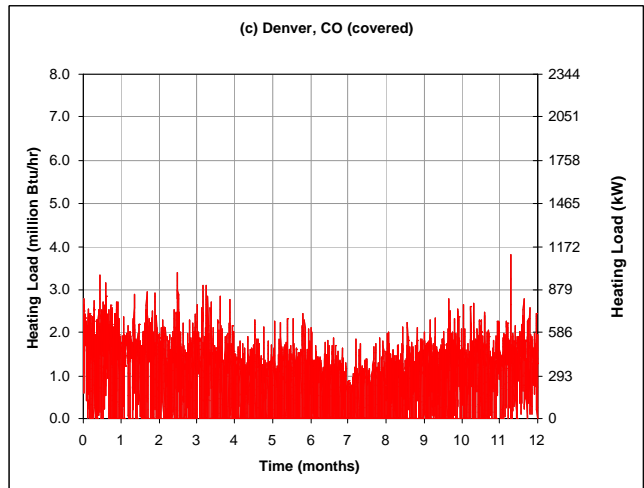
Figure 3. Hourly heating loads on an annual basis for covered aquaculture tanks.
