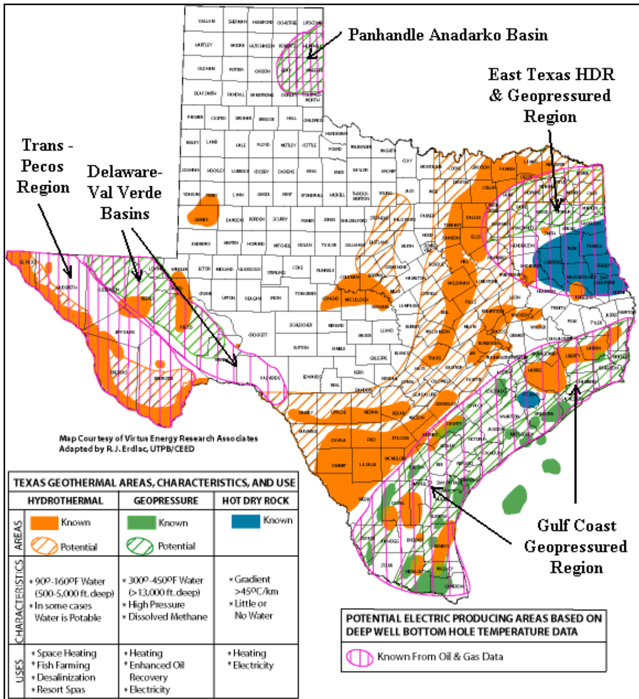
Texas geothermal resources as defined by the Texas Renewable Energy Resource Assessment of 1995. The location and boundaries of these geothermal areas are approximate. (The University of Texas of the Permian Basin)
