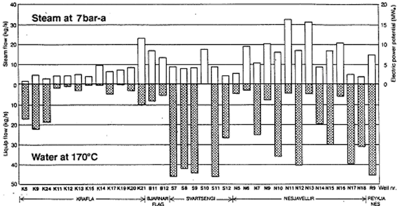
Figure 6. Typical Icelandic well yields.
