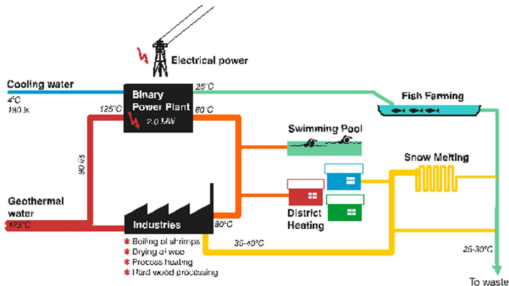
Figure 1. Húsavík, Iceland energy development.
