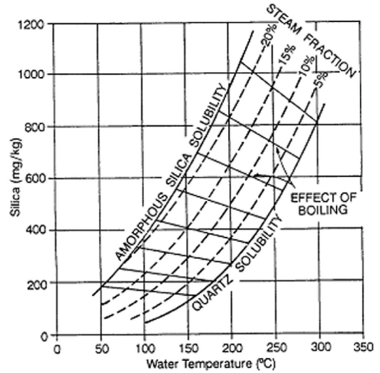
Figure 7. Solubility of silica.
