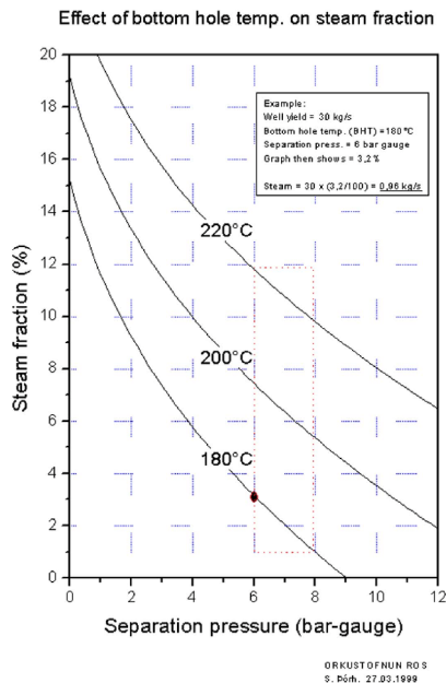
Figure 10. Fluid separation.
