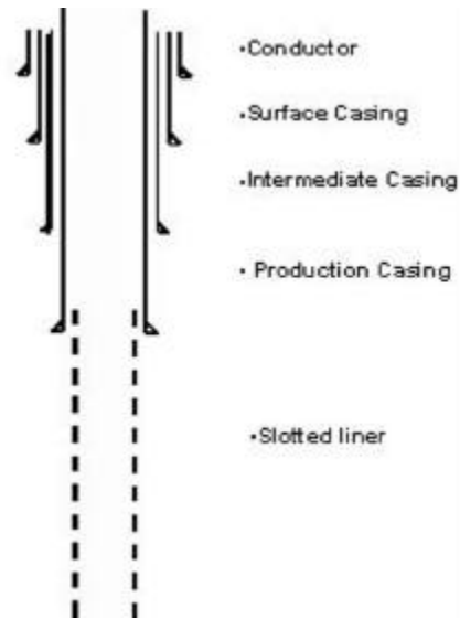
Figure 4. Casing types.
