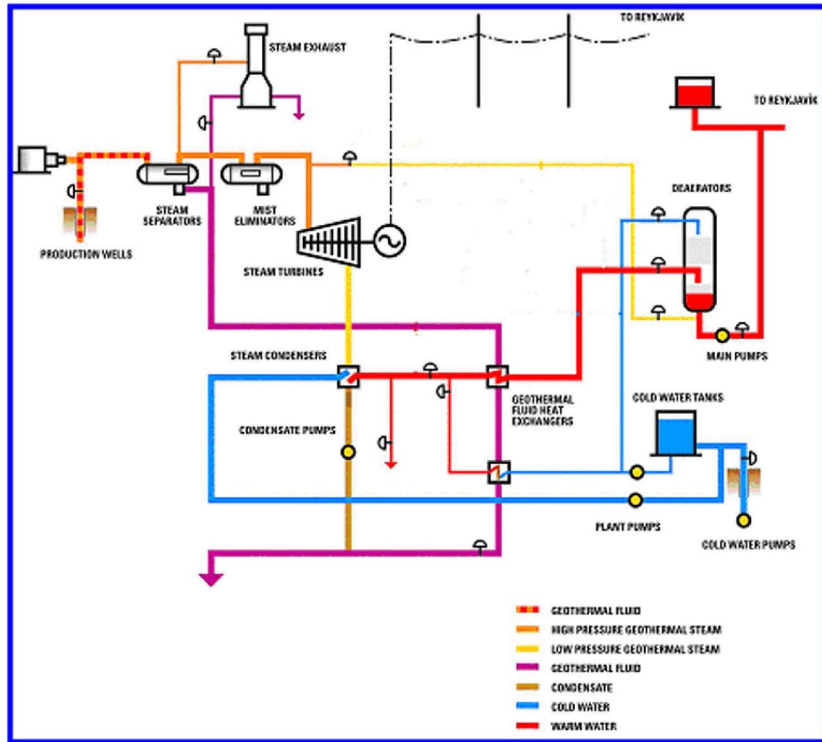
Figure 2. Nesjavellir, Iceland energy development.
