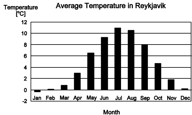
Figure 3. Average monthly temperatures in Reykjavik, Iceland.
