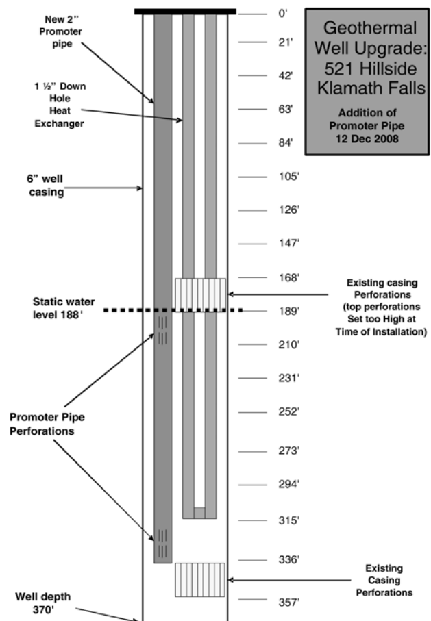
Figure 9: Schematic of System Two well.
