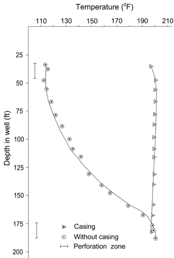
Figure 3: Temperature vs. depth for a geothermal well (with and without perforations).
