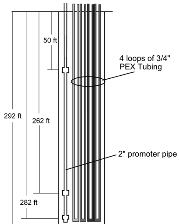
Figure 6: Schematic of System One well.
